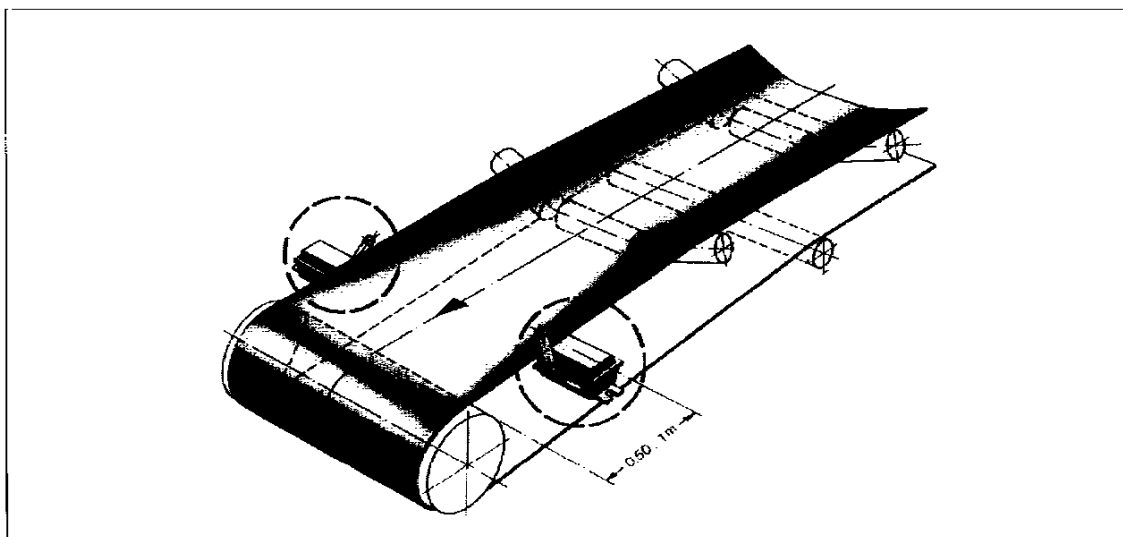
Mounting example BSR / BSO
